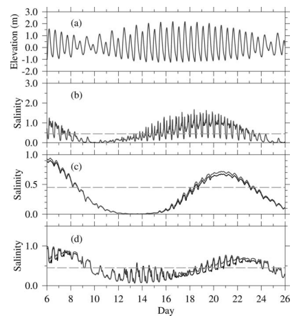
Figure 7. Modeled temporal variation of the elevation at the water intake of the Qingcaosha Reservoir (a) and the surface salinity at the water intakes of the Dongfengxisha Reservoir (b), Chenhang Reservoir (c), and Qingcaosha Reservoir (d) before and after the project from 6 February to 26 February in 2014. The dashed line is 0.45, which is the standard salinity of drinking water.
